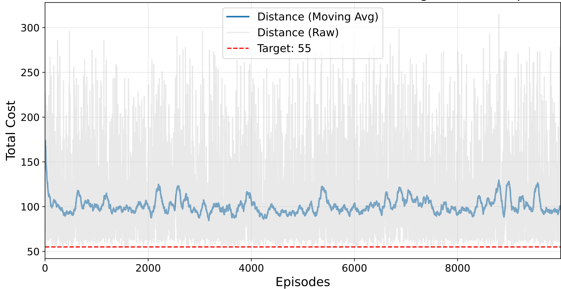
Final HYPERBAND GP Masked AutoRL-SOP Training - br17.12.sop
